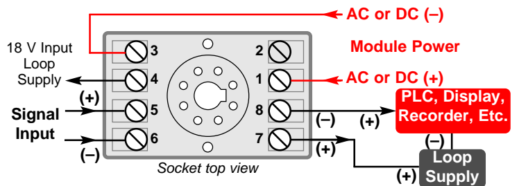
API 4300 G EXTSUP typical output wiring
