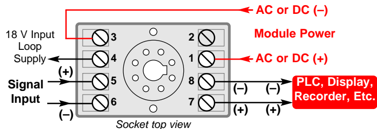
API 4310 G typical output wiring
