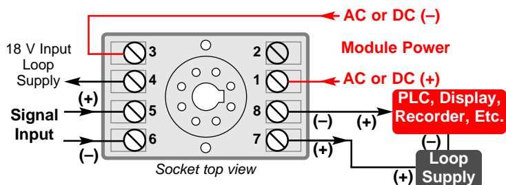
API 4310 G EXTSUP typical output wiring
