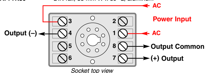
Socket top view API 9046-CH Bipolar Output Models
